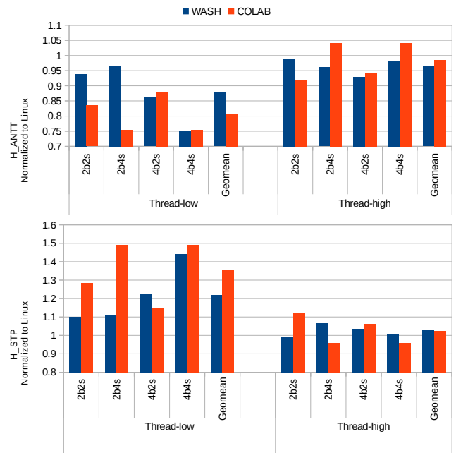
Figure 8. Performance of low number of application threads and high number of application threads Workloads. All results are normalized to the Linux CFS ones. Lower is better for H_ANTI and higher is better for H_STP.
