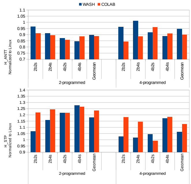
Figure 9. Performance of 2- and 4-programmed Workloads. All results are normalized to the Linux CFS ones. Lower is better for H_ANTI and higher is better for H_STP.
