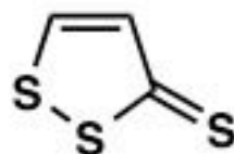
1,2-dithiole-3-thione (D3T)
