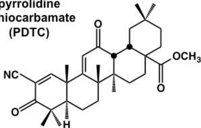
bardoxolone methyl
