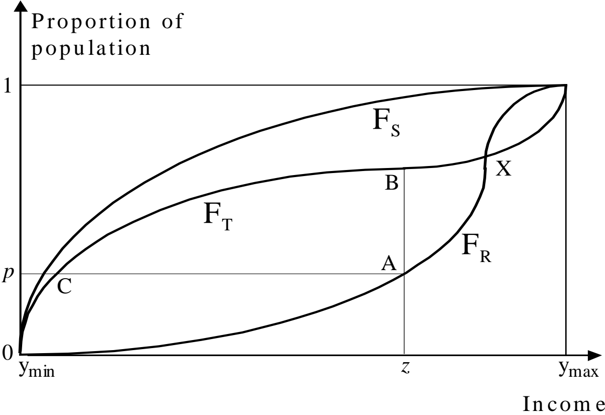
Figure 1. Cumulative distribution functions (illustrating stochastic dominance relationships)
