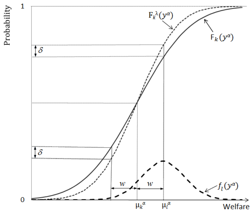
Figure 1b. Graphical proof of the identification property
