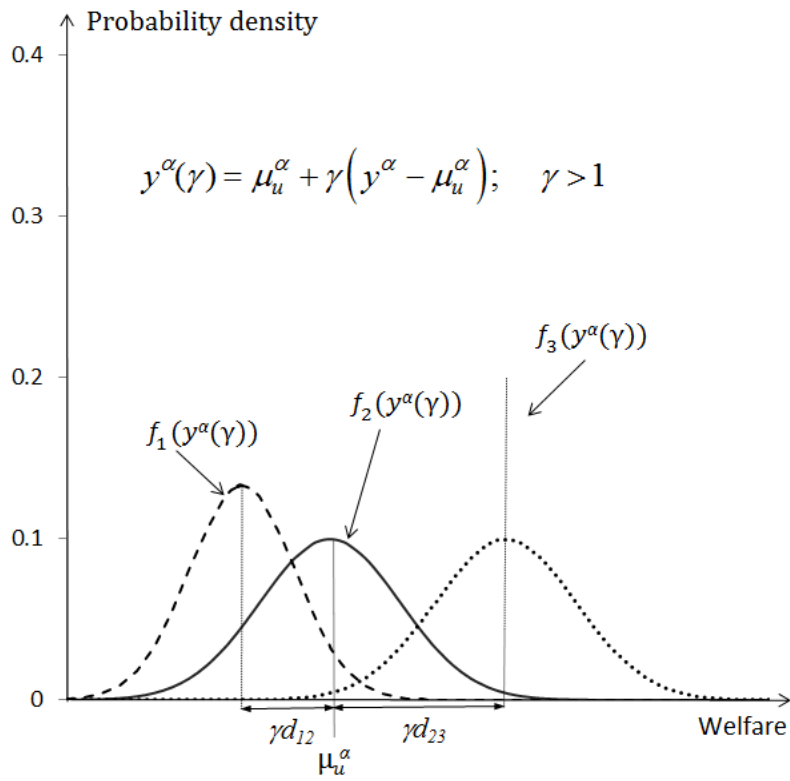
Figure 2. Illustration of alienation axiom
