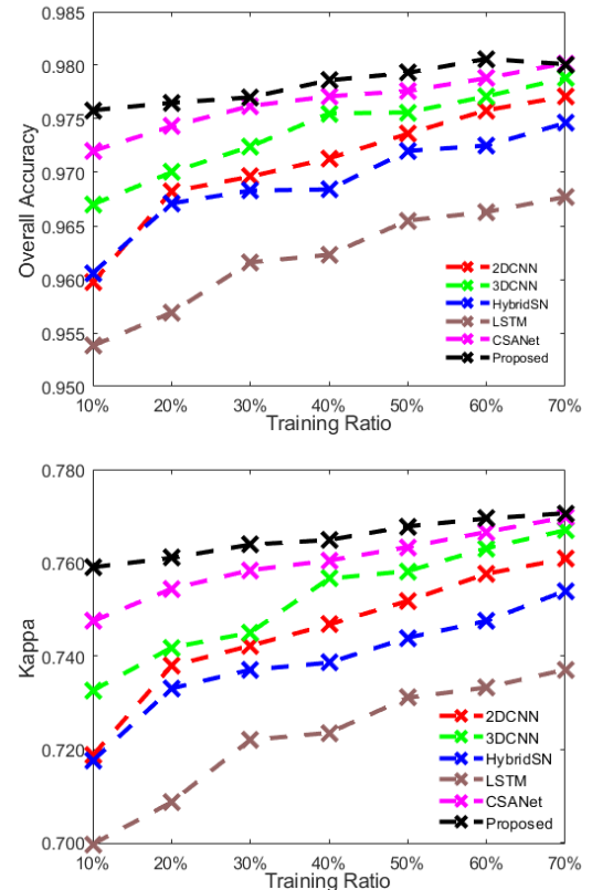
Fig. 6. Comparing the OA (top) and KP (bottom) results of all DL methods on the River dataset under different training ratios.
