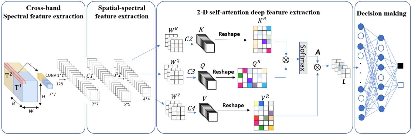
Fig. 1. The architecture of the proposed CBANet model
