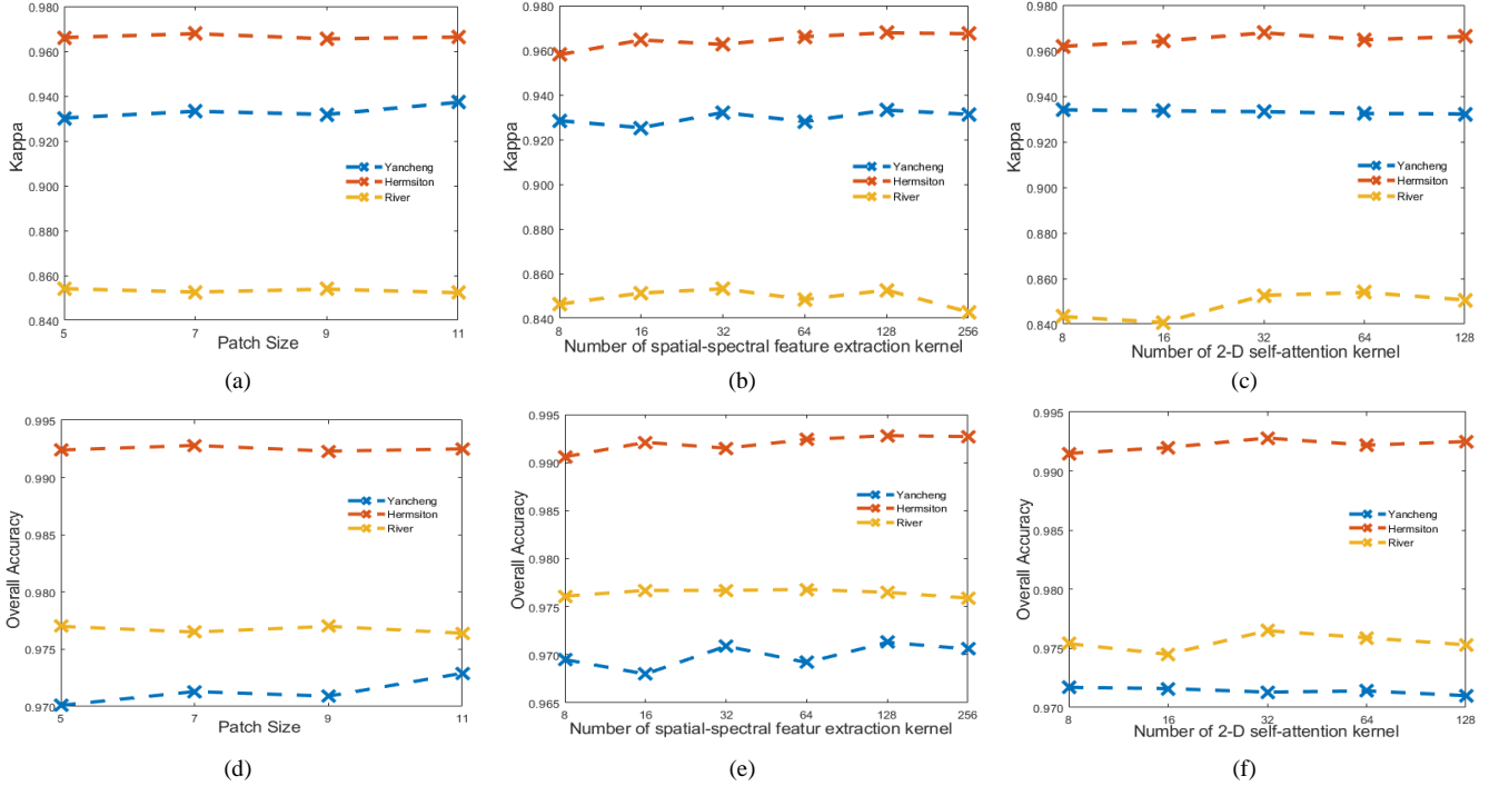
Fig. 7. Ablation experiments and results of the CBANet in different settings on the three datasets, including the Kappa values of different patch sizes (a), different number of spatial-spectral feature extraction kernel (b), and different number of 2D self-attention kernel (c), as well as the OA values under different patch size (d), different number of spatial-spectral feature extraction kernel (e), and different number of 2D self-attention kernel (f).
