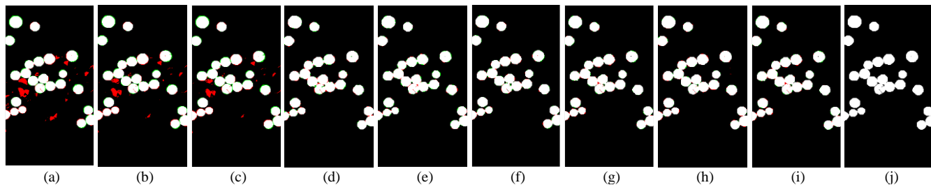
Fig.5. Extracted change maps on the Hermiston Dataset from different methods of AD (a), CVA (b), PCA-KM (c), LSTM (d), HybridSN (e), 3-DCNN (f), 2-DCNN (g), CSANet (h) and CBANet (i) in comparison to the Ground-truth map (j), where the false alarms and missing pixels are labelled in red and green.
