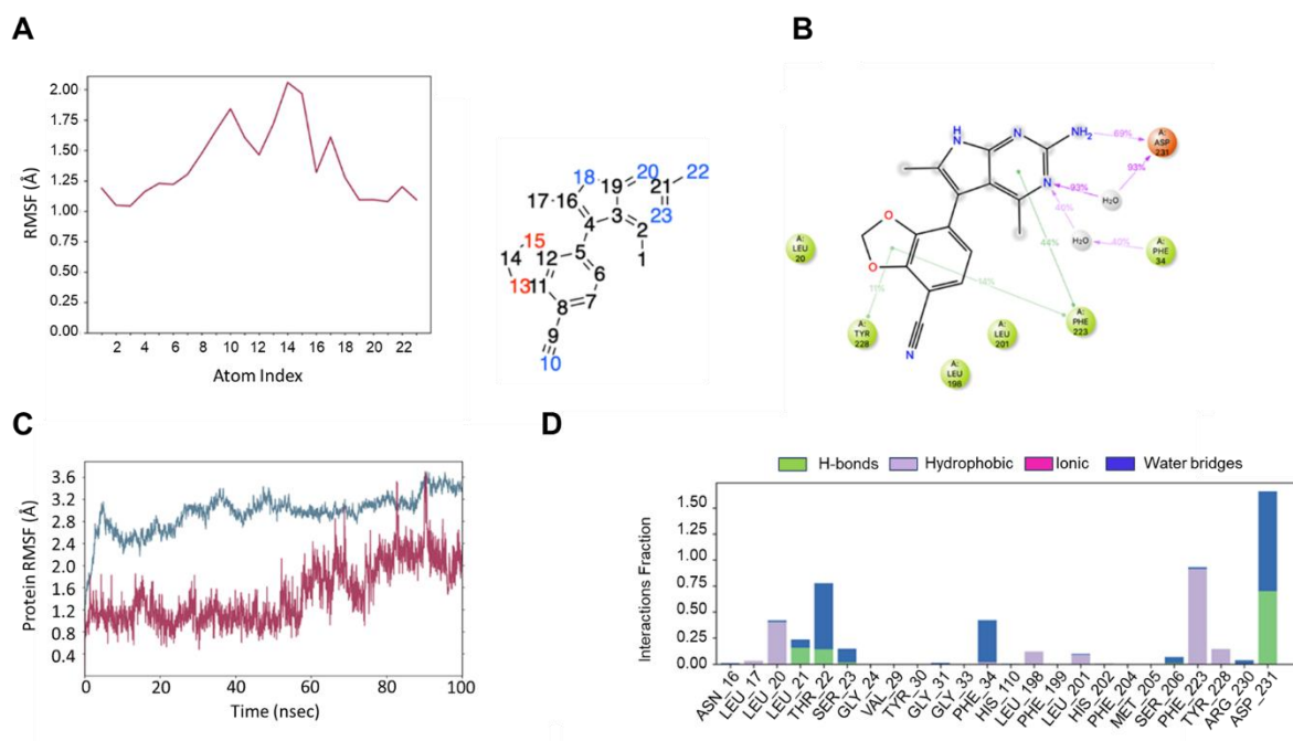
Fig. S3 (A) The Ligand Root Mean Square Fluctuation (RMSF) for each atom of DNDI-6174 in cytochrome b (wild-type) measuring the changes in the position of ligand atoms during the 100 ns MD simulation (atom number as reported in the chemical representation on the right). These studies indicate that benzodioxole moiety of DNDI-6174 is the portion of the molecule with the highest flexibility during binding. (B) A schematic of detailed ligand atom interactions with the amino acid residues of cytochrome b . (C) Root Mean Square Deviation (RMSD) plot of DNDI-6174 (right Y-axis – magenta curve) and wild-type cytochrome b (left Y-axis – blue curve). The plot indicates the stability of the protein and the ligand during the simulation. The overall stability of the docking binding pose is highlighted by the protein and ligand RMSD over this simulation. (D) Protein-Ligand Contacts plot. The possible interactions are categorized into four types: hydrogen bonds, hydrophobic, ionic and water bridges. The stacked bar charts are normalized over the course of the trajectory.
