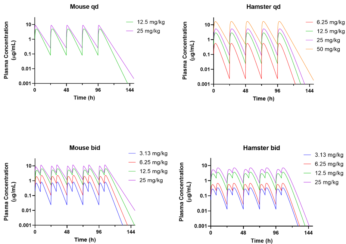
Fig. S13 Simulated repeat dose plasma profiles for DNDI-6174 in mice and hamsters following once or twice-daily oral administration (8 and 24 h) for 5 days as used in the efficacy studies.
