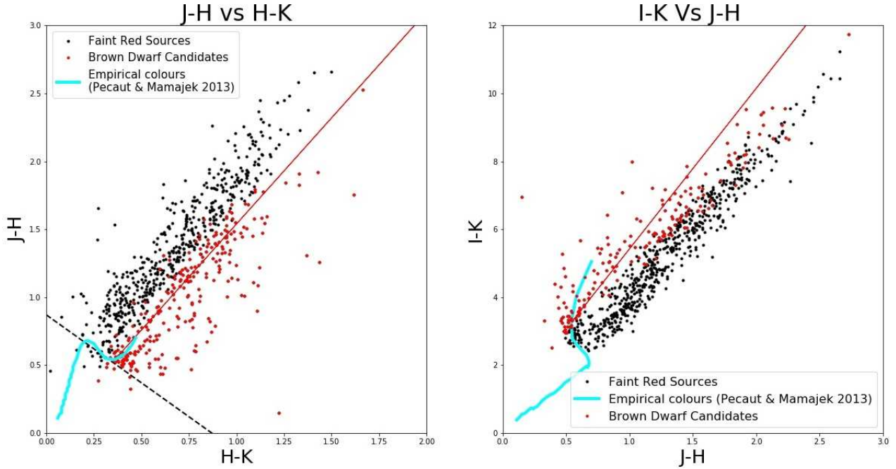
Figure 9. Two infrared colour-colour plots showing the 902 faint red sources identified in at least one of the samples: DISCS, KINEMATIC, HIGHEX & VAR. The red lines indicate M6 extinction vectors. The extinction law was taken from Mathis (1990) ( R_V = 3.1 ), the empirical colours are from Pecaut & Mamajek (2013). Sources falling in the expected regions for substellar objects, with their associated error bars, were selected as brown dwarf candidates. The dashed black line in the left plot is the approximation of the empirical colour sequence for young stars, used for extinction estimation.
