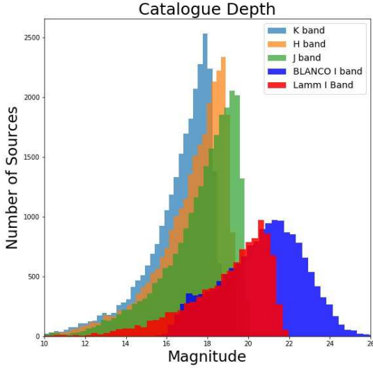
Figure 3. A histogram of the I-band magnitudes of the BLANCO and the Lamm catalogue, as well as the JHK magnitudes in the BASE catalogue.
