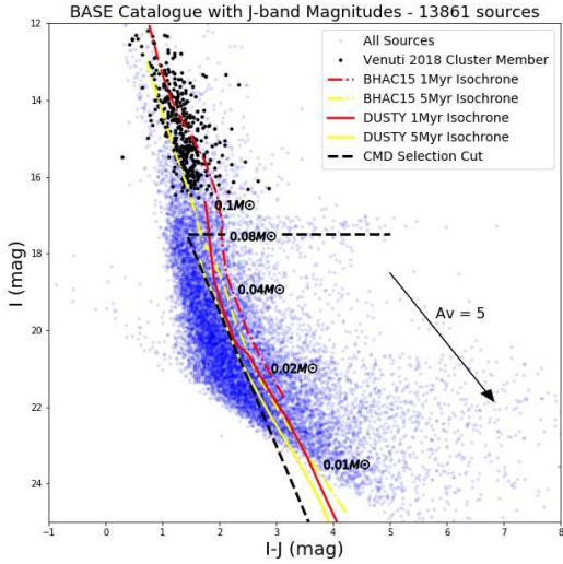
Figure 5. I vs I-J colour magnitude diagram for the BASE catalogue, overplotted with known cluster members and 1 & 5 Myr BHAC15 & DUSTY isochrones. An approximate mass scale is labelled in black. The straight line cutoff at the faint end of the catalogue is due to the limiting depth of the FLAMINGOS catalogue.
