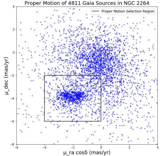
Figure 6. The proper motions of 4811 sources within NGC2264. The smaller cluster of sources is NGC2264, the black box indicates the proper motion selection criteria.
