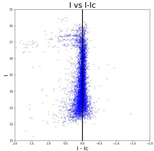
Figure 2. A comparison between the Lamm catalogue and our calibrated Blanco
