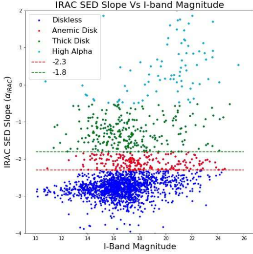
Figure 7. The slope of the Spitzer/IRAC SED \alpha_{IRAC} vs. I-band magnitude. The cuts used to differentiate between disc bearing and discless sources are taken from Lada et al. (2006).
