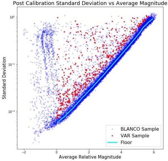
Figure 4. A plot comparing the average magnitude and standard deviation of each source over the 221 images, after the differential photometry and calibration.
