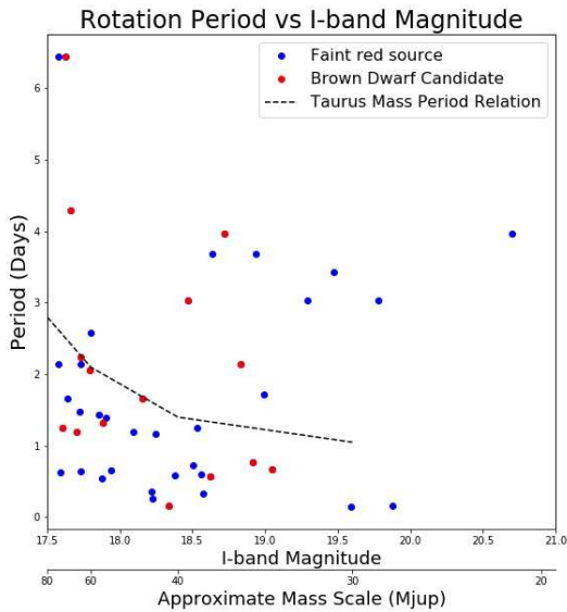
Figure 13. I-band vs. rotation period. The dashed black line indicates the period-mass relation found in Taurus by (Scholz et al. 2018)
