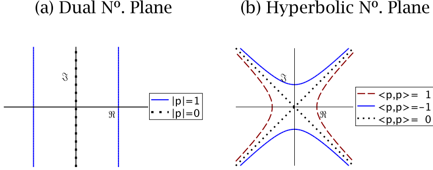
Figure 1: Unit length and zero divisors hyperbolic and dual numbers: (a) Dual numbers zero divisors (dotted black line), and unit length dual numbers (solid blue line). A unit length dual number may be written as (\pm 1, \phi) \mapsto \pm 1 + \phi \varepsilon ; (b) Hyperbolic numbers zero divisors (dotted black line), and unit length hyperbolic numbers (solid blue and dashed red lines). There exist four types of unit length hyperbolic numbers, the dashed red lines correspond to (\pm \cosh \phi, \sinh \phi) \mapsto \pm \cosh \phi + \ell \sinh \phi and the solid blue lines correspond to (\sinh \phi, \pm \cosh \phi) \mapsto \sinh \phi \pm \ell \cosh \phi . In particular, the dashed red line for \Re > 0 corresponds to O^{++}(2) , the group of time orientation preserving hyperbolic rotations (see Subsect. 6.1.)
