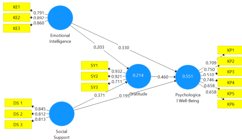
Figure 2. Alogarithm results
