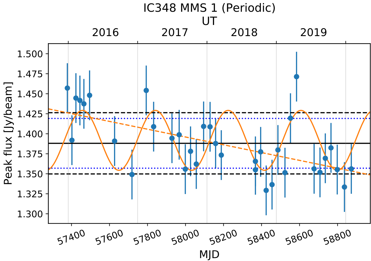
Figure B.1. Light curve of the identified variable source, MMS 1 in IC 348. Black solid line indicates the mean peak brightness in \text{Jy beam}^{-1} . Black dashed line and blue dotted line indicate the observed standard deviation and fiducial error from the mean peak brightness, respectively. The orange solid line denotes the sinusoidal fitting provided by LSP while the orange dashed line denotes the linear fitting result. Both the linear and sinusoidal fits are robust, \text{FAP} < 0.1\% . See Tables 3 and 4 for details.
