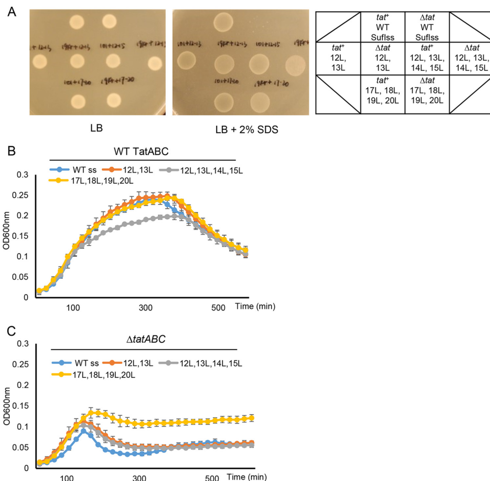
FIG 7 Multiple leucine substitutions in SufI signal peptide h-region partially reroute AmiA to the Sec pathway. Overnight cultures of strain MC4100 \Delta amiA \Delta amiC \Delta tat ABC harboring either pTH19kr ( Δtat ) or pTAT101 producing wild-type (WT) TatABC ( tat + ) along with pSUSufI ss -mAmiA producing the indicated substitutions in the SufI signal peptide were subcultured at a 1:100 dilution. (A) Cultures were grown for a further 3 h at 37°C, pelleted, and resuspended to an OD 500 of 0.1, and 8 μl of sample was spotted onto LB agar or LB agar containing 2% SDS. Plates were incubated at 37°C for 16 h. (B and C) Alternatively, cultures were supplemented with 0.5% SDS (final concentration) and grown at 37°C without shaking. The optical density at 600 nm was monitored every 20 min using a plate reader. Error bars are ±standard deviations ( n = 3 biological replicates).
