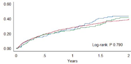
Kaplan-Meier failure estimates
