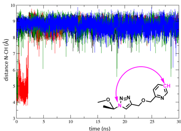
Figure 5. Molecular dynamics of 10 showing unfolding after 2.5 ns and its maintenance up to 30 ns. Starting structures: red trace: protonated folded; green trace: neutral folded; black trace: protonated unfolded; blue trace: neutral unfolded
