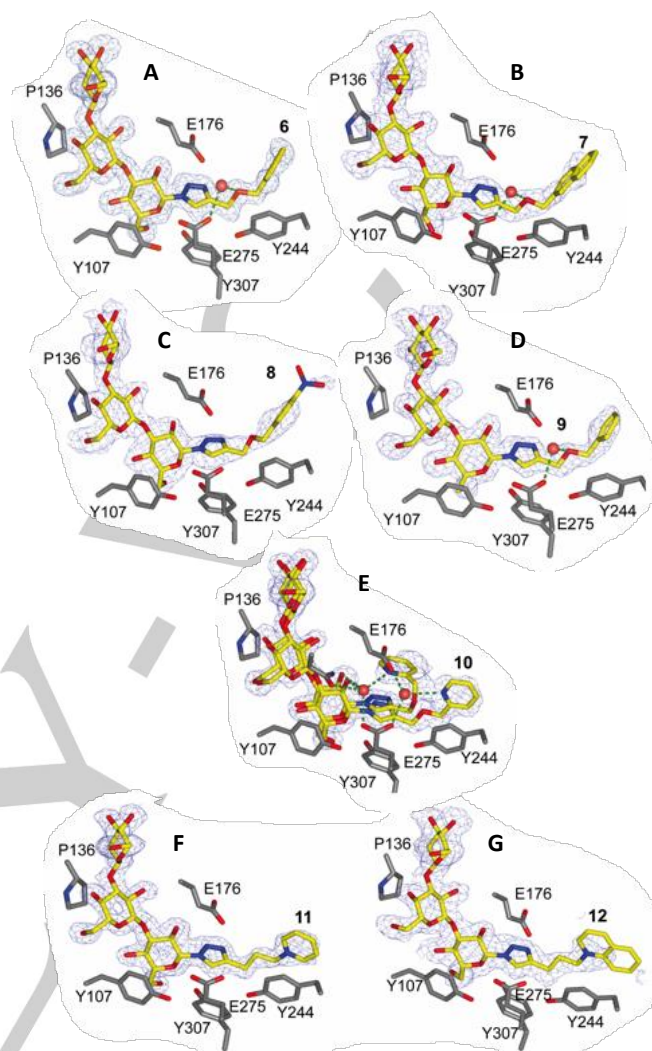
Figure 4. X-ray structures of ScGas2 in complex with 6 (A), 7 (B), 8 (C), 9 (D), 10 (E), 11 (F) and 12 (G). The unbiased (i.e. before inclusion of any ligand model) |F_o| - |F_c| , \phi_{\text{calc}} electron density maps are shown at 2.2 \sigma .
