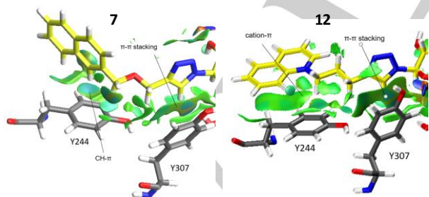
Figure 6. NCI analysis showing characteristic surfaces for T-shape (left, compound 7 ) and parallel (right, compound 12 ) oriented ligands corresponding to CH- \pi and azinium- \pi (cation- \pi ) interactions, respectively.
