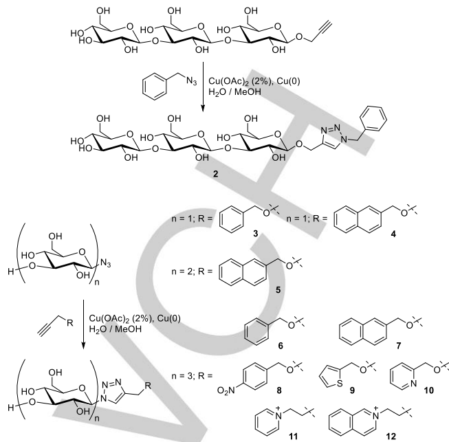
Figure 2. Chemical synthesis of ligands through typical click-chemistry.
