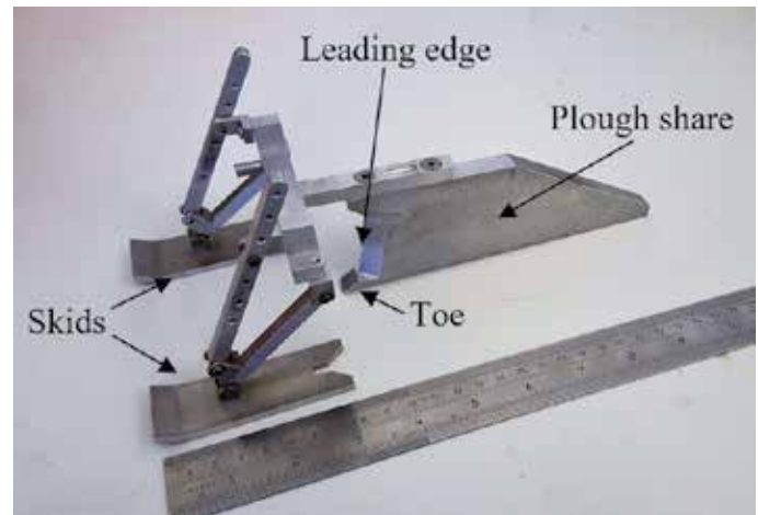
Figure 1: 1/50 th scale seabed cable plough
