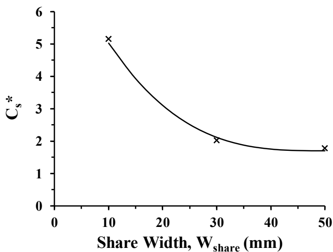
Figure 9: Variation of C_s^* with share width at D_r = 50\%
