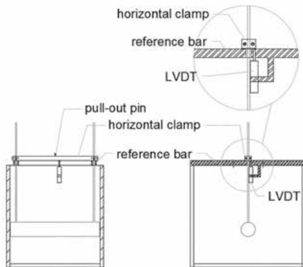
Figure 2 Flotation and pull-out test setup: (a) side view; (b) frontal view with detail of the reference bar detail shown expanded.
