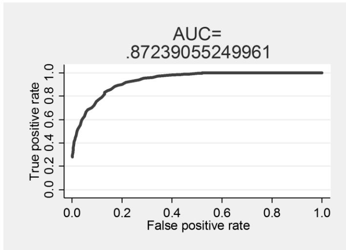
Figure 2a. ROC curves of symptom dimensions used in the prediction of B-SNIP biotypes
