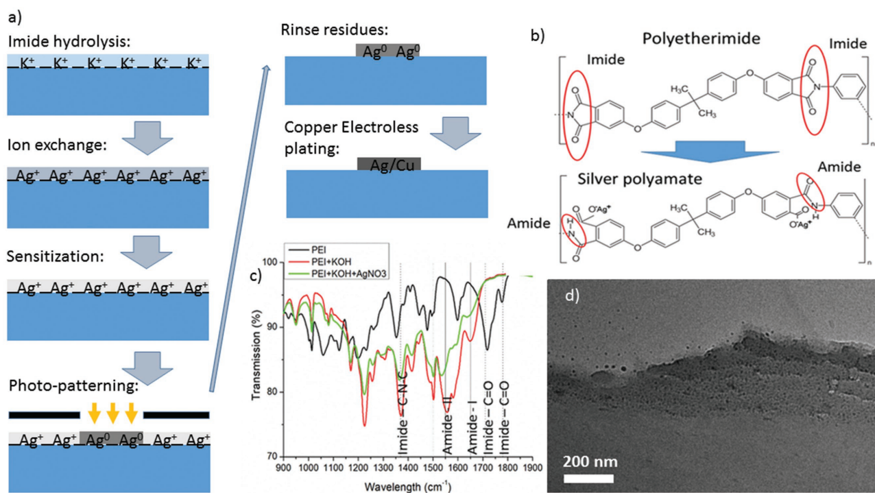
Figure 1. a) Process to achieve the metallization of polyimide and polyetherimide. The sensitization step is crucial to achieve a fast process. b) Hydrolysis breaking of the imide ring. Potassium ion was replaced by silver using ion exchange, which produced silver polyamate. c) FTIR of the PEI at different stages of the process. d) TEM cross-section of ULTEM 9085 treated sample revealing the NPs on its surface.
