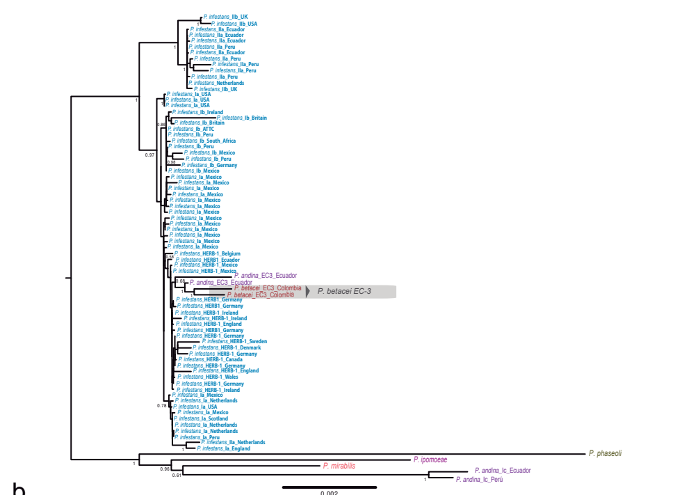
Fig. 1 Phylogenetic relationships of the Phytophthora betacei isolates and the closely related species, based on genotyping by sequencing (GBS) data and phylogeny of complete mitochondrial genomes. a. The tree was inferred using maximum likelihood (ML) with P. phaseoli as an outgroup. Support values associated with branches correspond to ML bootstrap support values (BS); b. ML phylogeny of complete mitochondrial genomes showing the phylogenetic position of P. betacei sp. nov. Only bootstrap support values above 50 % are shown.
