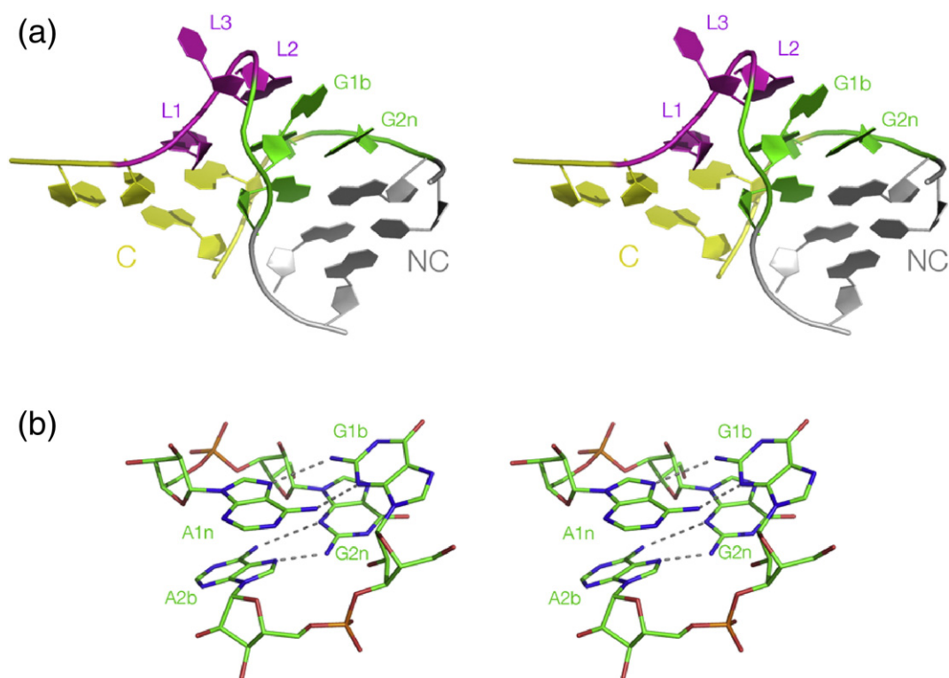
Fig. 2. The overall structure of the k-turn, and the G·A pairs at the core. Parallel-eye stereoscopic images are shown. (a) The k-turn structure shown in cartoon form. (b) The two trans sugar-Hoogsteen G·A pairs. Note that the minor groove edges of the adenine bases are oriented leftward in this view, that is, are directed toward the minor groove of the C helix.
