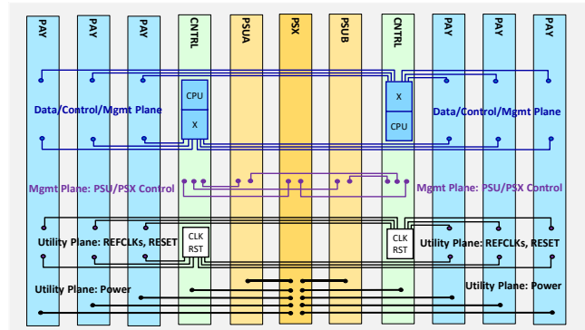
Figure 7: Proposed SpaceFibreVPX Backplane
