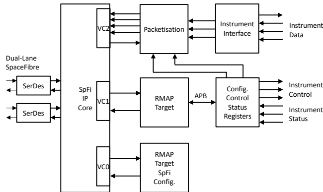
Figure 1: Dual-Lane SpaceFibre Instrument Interface
