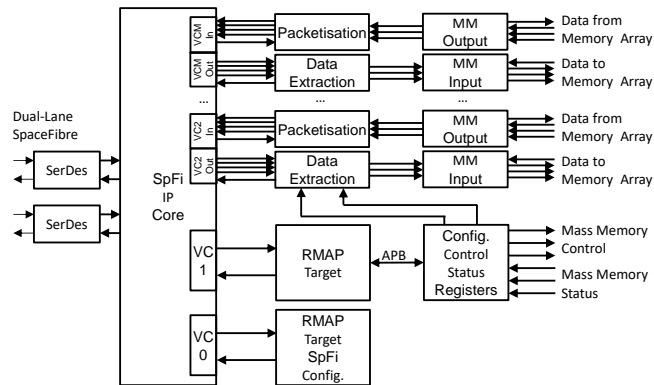
Figure 4: Dual-Lane SpaceFibre Mass-Memory Interface
