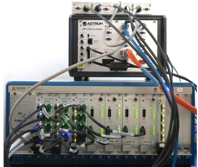
Figure 5: Prototype Next Generation Mass Memory System
