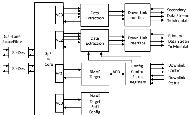
Figure 6: Dual-Lane SpaceFibre Downlink Interface
