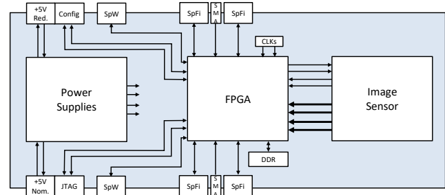
Figure 2: SpaceFibre Camera Block Diagram
