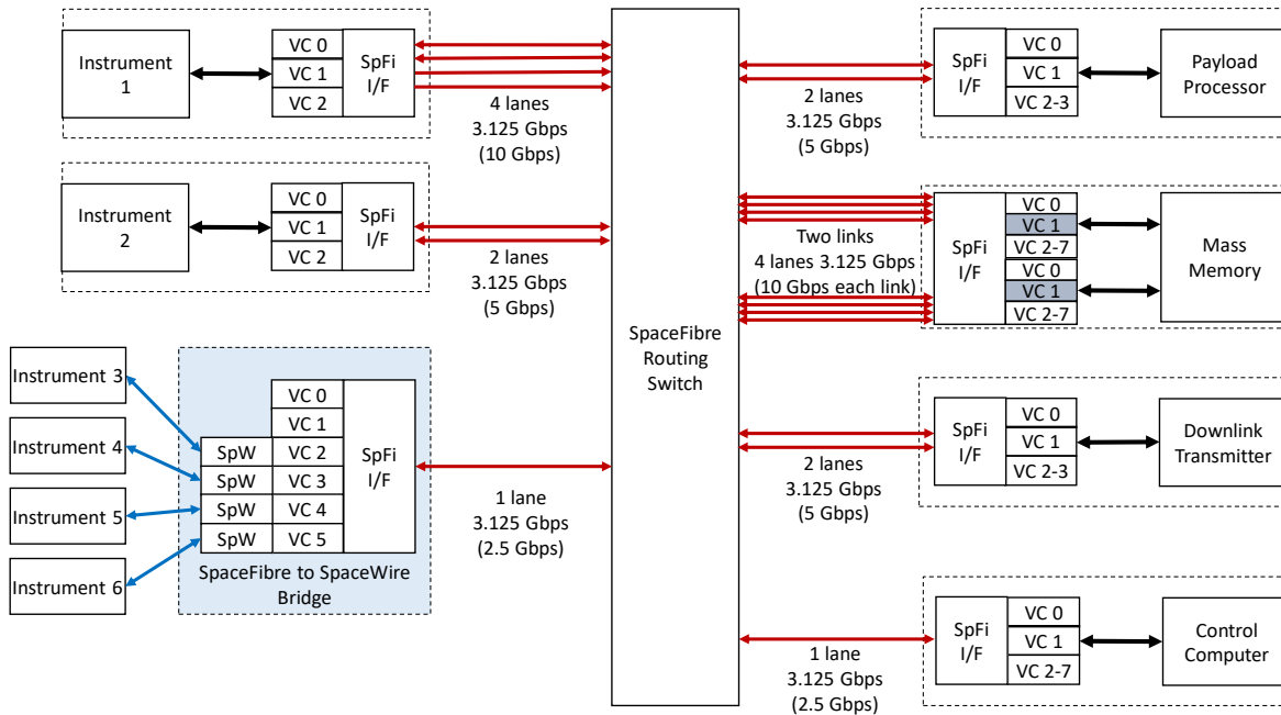
Figure 8: Example SpaceFibre Payload Data-Handling Network
