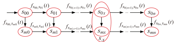
Fig. 5. State transition diagram for interconnected GPs.
