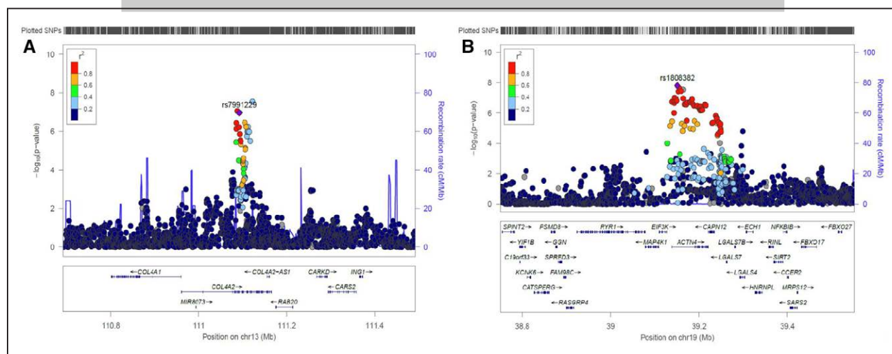
Figure 3. Regional association and recombination plots of variants that reached genome-wide significance in overall meta-analysis (discovery and replication stage).
