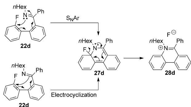
Scheme 7. Two putative mechanisms for the formation of phenanthridinium salt 28d from N -alkylimine 22d differing in the mode of cyclisation to give Meisenheimer complex 27d .
