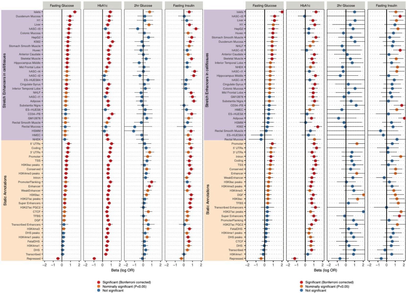
A. GWAS P value threshold = 1e-05
