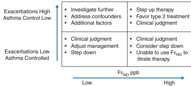
Figure 2. Conceptual framework for the use of fractional exhaled nitric oxide ( F_{E_{NO}} ) testing to guide treatment decisions for individuals with asthma. The decision to act on an individual F_{E_{NO}} value in an individual patient requires that the clinician combine clinical judgments based on the perceived probability of benefit, with particular attention being given to the key outcome measures such as exacerbation risks that were assessed in this guideline. As the level of F_{E_{NO}} increases in value, the specificity for a step up in therapy increases, whereas accepting lower values of F_{E_{NO}} to make treatment decisions places a higher value on the sensitivity to detect the possibility that a step up in therapy may impact asthma control.
