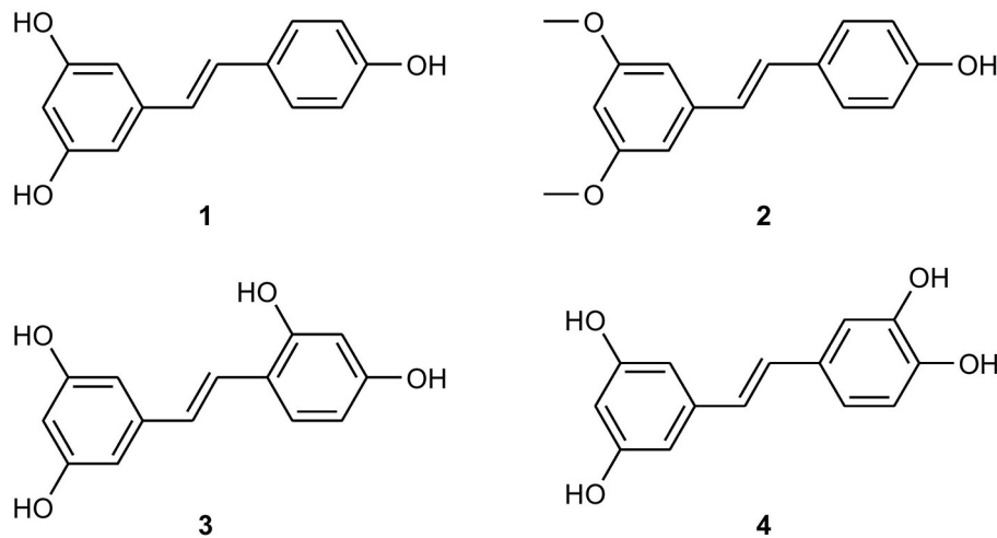
FIGURE 1 | Chemical structures of (1) resveratrol (2) pterostilbene (3) oxyresveratrol (4) piceatannol.
