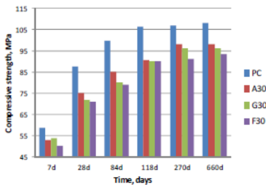
Figure 2. The evolution of compressive strength of mortar specimens, at 30% soda-lime WGP's substitution for PC
