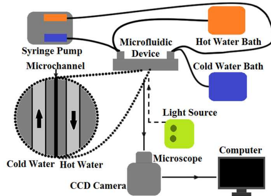
Figure 2. The experimental setup for the thermophoresis investigation. The microfluidic device consists of two larger channels for keeping temperature difference and one central sample microchannel.
