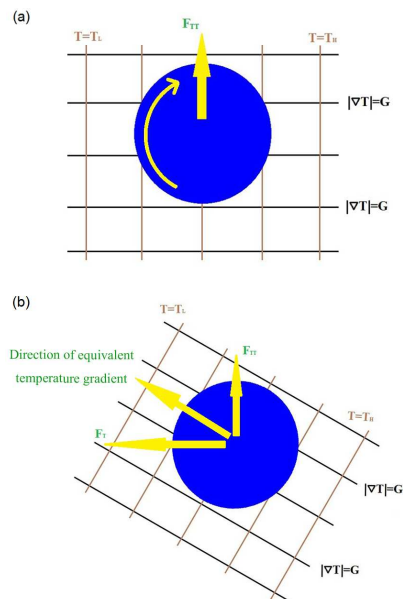
Figure 1. Spherical particles in the fluid with uniform temperature gradient. The particle is rotating in the fluid. (a) The thermophoretic tension force exerted on a rotating particle, where |\nabla T| is the magnitude of temperature gradient and F_{TT} is the thermophoretic tension force. (b) The thermophoretic related force exerted on a particle in the equivalent temperature field, where F_T represents the thermophoretic force.
