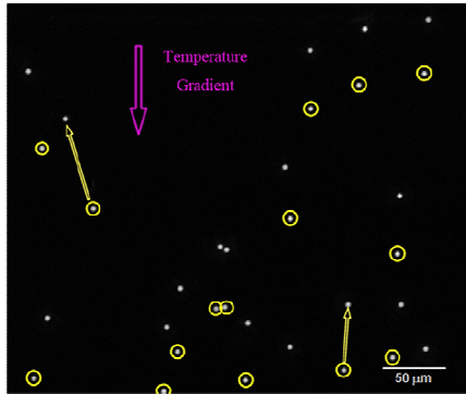
Figure 3. Particle movement in microchannel under temperature gradient.
