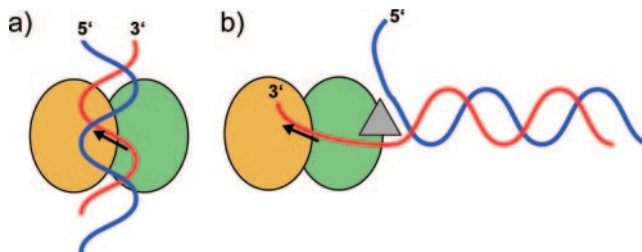
Figure 2. Unified mechanism of Snf2 family ATPases and DExx box helicases. Schematic comparison of (A) dsDNA translocases (e.g. Snf2) and (B) ssDNA translocases (e.g. PcrA and NS3 helicases). Both enzyme families contain a conserved RecA-like domain core (orange/green), but differ in other subunits (data not shown). Helicases transport product ssDNA and often contain an upstream DNA unwinding element (grey triangle). In contrast, Snf2 family enzymes also recognize the 5'–3' strand (blue) and track along the minor groove. Despite many functional differences, however, both enzymes families bind the 3'–5' strands at an equivalent site across the two RecA-like domains, indicating that ATP-driven conformational changes transport DNA substrates via the 3'–5' strands in analogous ways (arrows).
