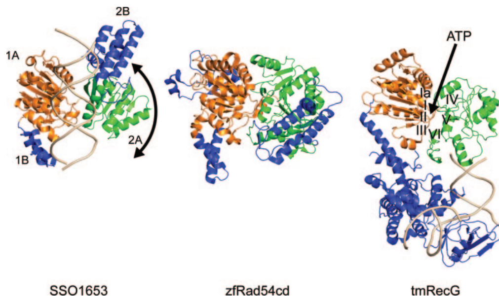
Figure 1. Comparison of Structures of Snf2 family enzymes and the RecG helicase. Structural comparison of the S.solfataricus (sso) SSO1653 catalytic domain [cd, (43), the zebrafish (zf) Rad54 cd (68) and T.maritima (tm) RecG (53). The three crystal structures are shown as ribbon models with highlighted secondary structures. DNA molecules bound to SSO1653 and tmRecG are shown as brown ribbon model. The two RecA-like domains (1A: orange, 2A: green) are shared across DExx box ATPases, and form the ATP-binding site in their interface cleft. The location of the ATP-binding site, as well as locations of the seven conserved helicase-related ATPase/DNA-binding motifs (Ia,II,III,IV,V,VI) are indicated in tmRecG. The two RecA-like domains interact with additional domains (1B and 2B: blue) that are suggested to convert ATP-driven rearrangements of 1A and 2A into the translocase or DNA unwinding function. For instance, these domains bind to the replication fork substrate in RecG, which is dragged like a plough through DNA by the action of the translocase module. The role of the helical domains of Snf2 family enzymes is not as well understood, but they could play a role in advancing the enzyme by ATP-driven conformational changes. Note that domain 2 of SSO1653 (2A and 2B) is flipped by 180° with respect to more typical conformations found in zfRad54cd and RecG (double arrow). This flip could represent an open conformation during substrate uptake.
